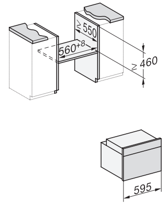
built-in H7000 M build-under, installation drawing
